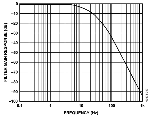
Figure 45. 10 Hz Sallen Key Low-Pass Filter
