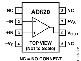
Figure 2. 8-Lead SOIC_N and 8-Lead MSOP
